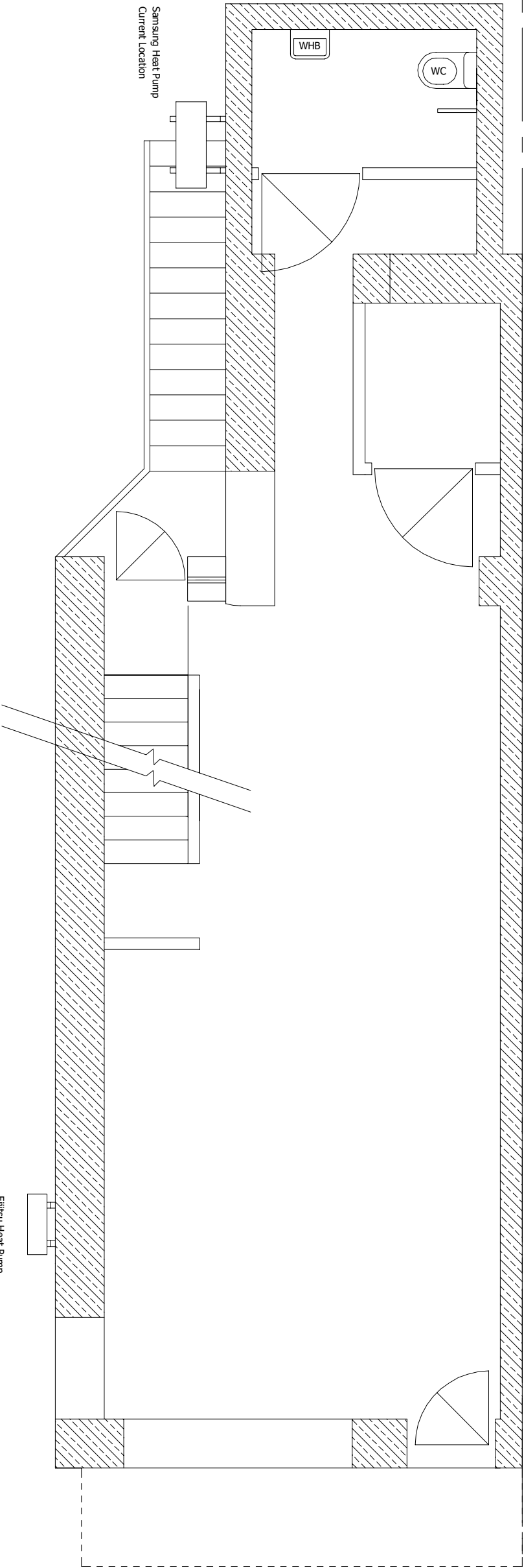
Ground Floor 1:50
