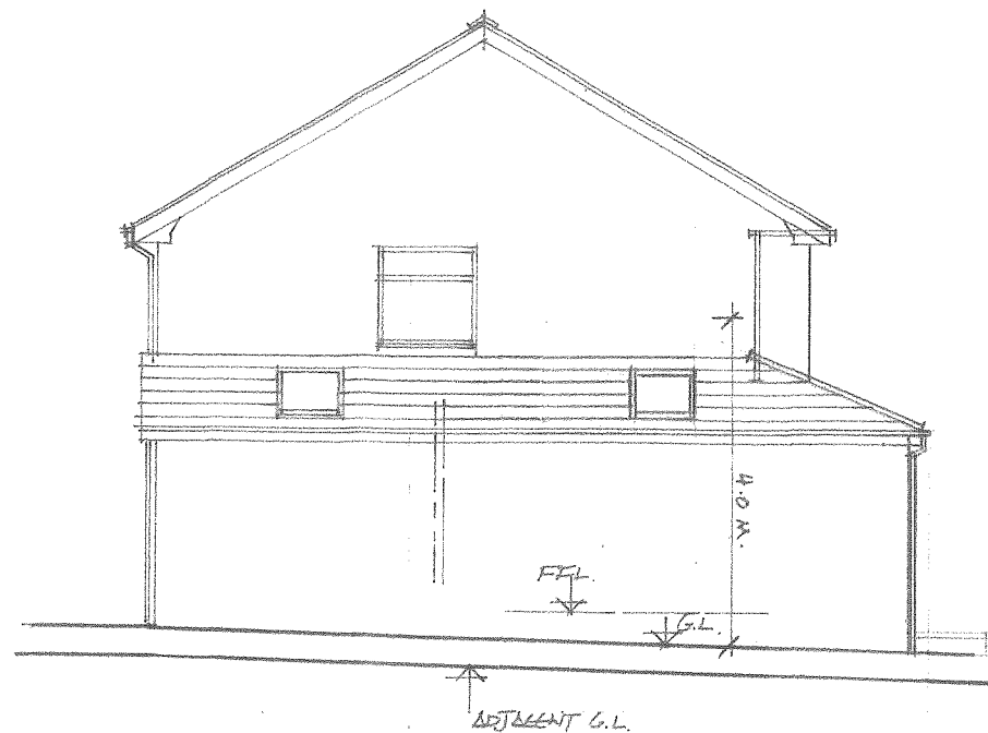
SIDE ELEVATION / S.E.
