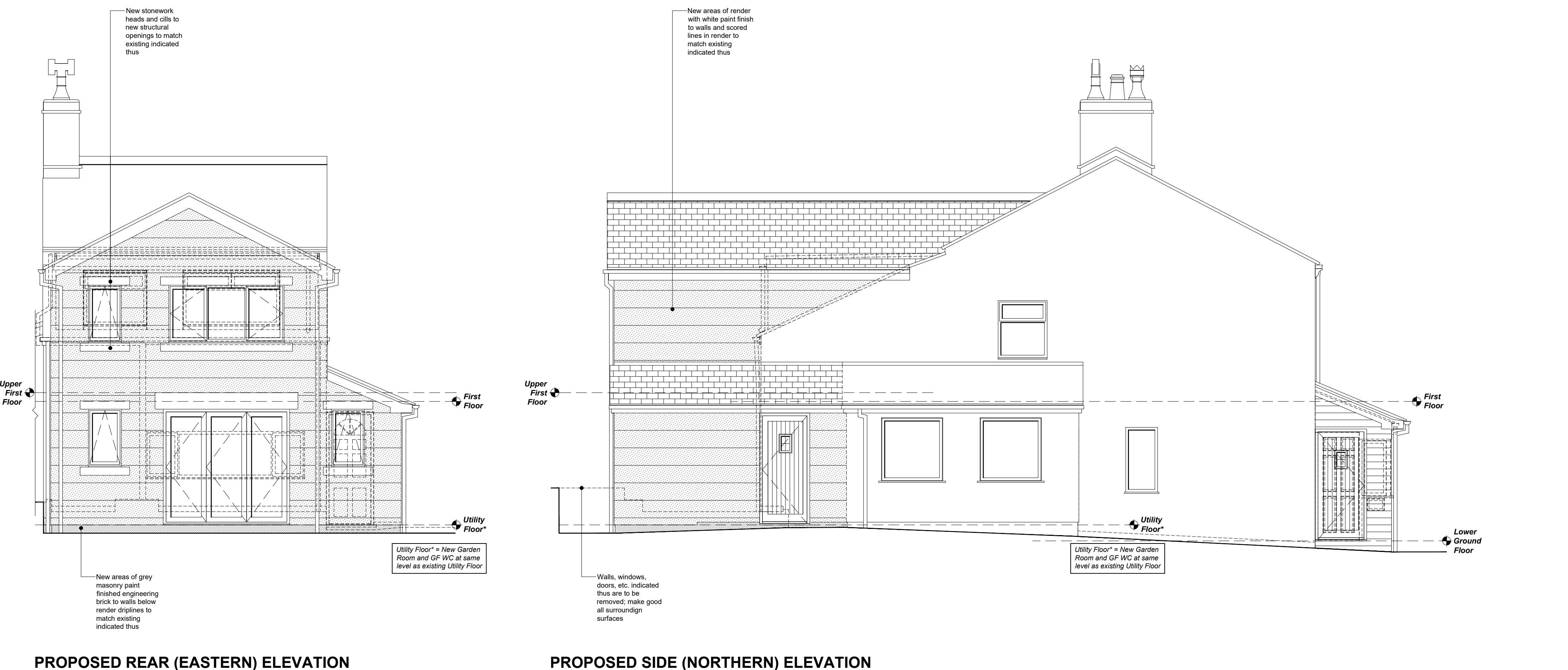
PROPOSED REAR (EASTERN) ELEVATION
