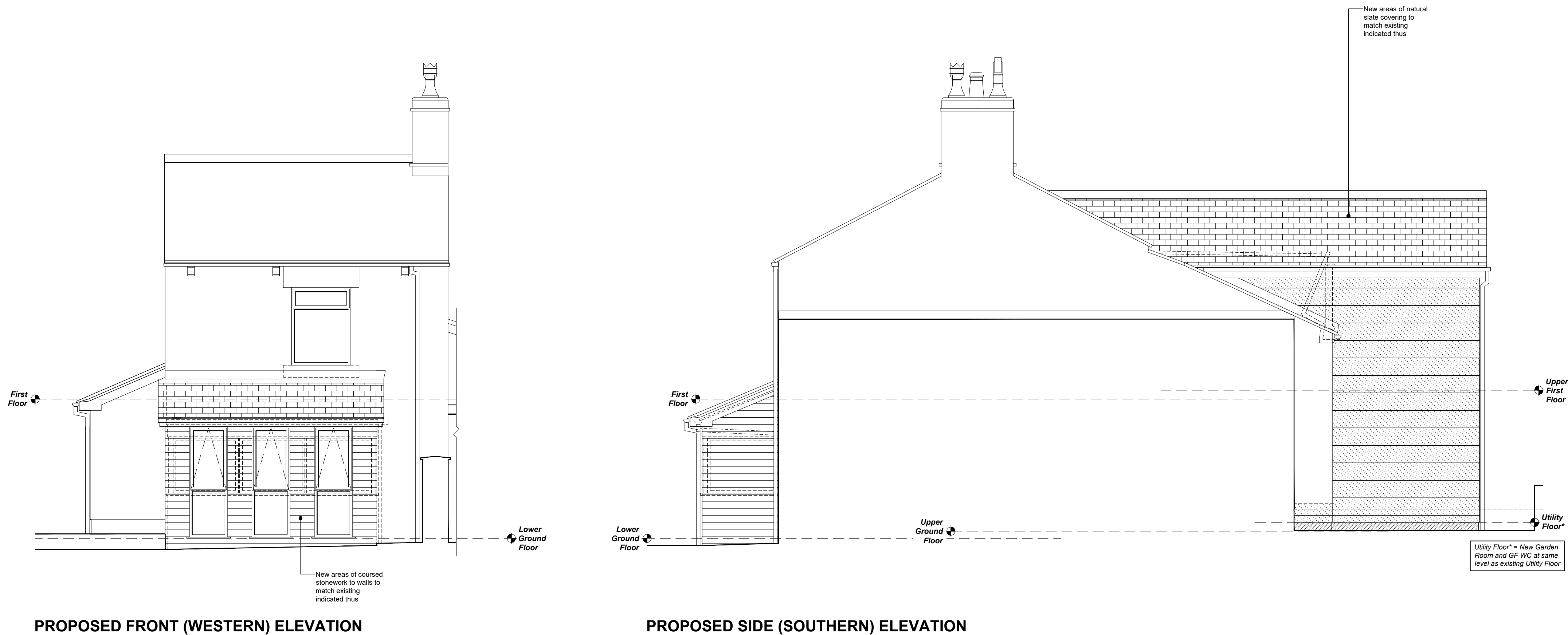
PROPOSED FRONT (WESTERN) ELEVATION
