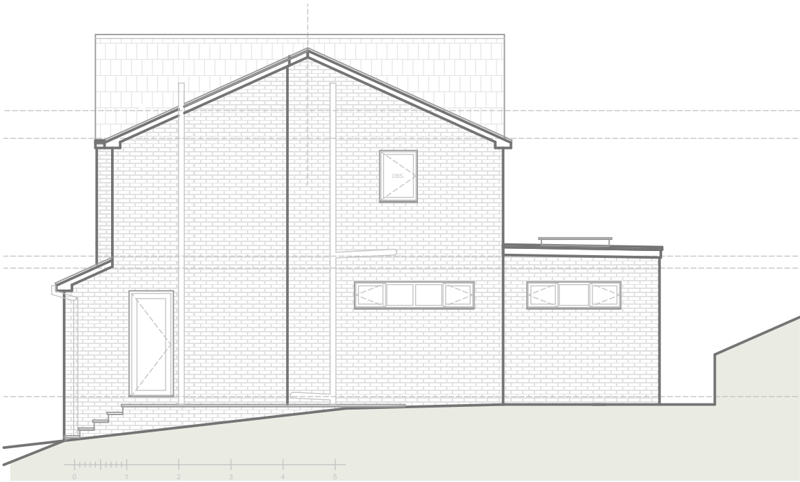
North Elevation
