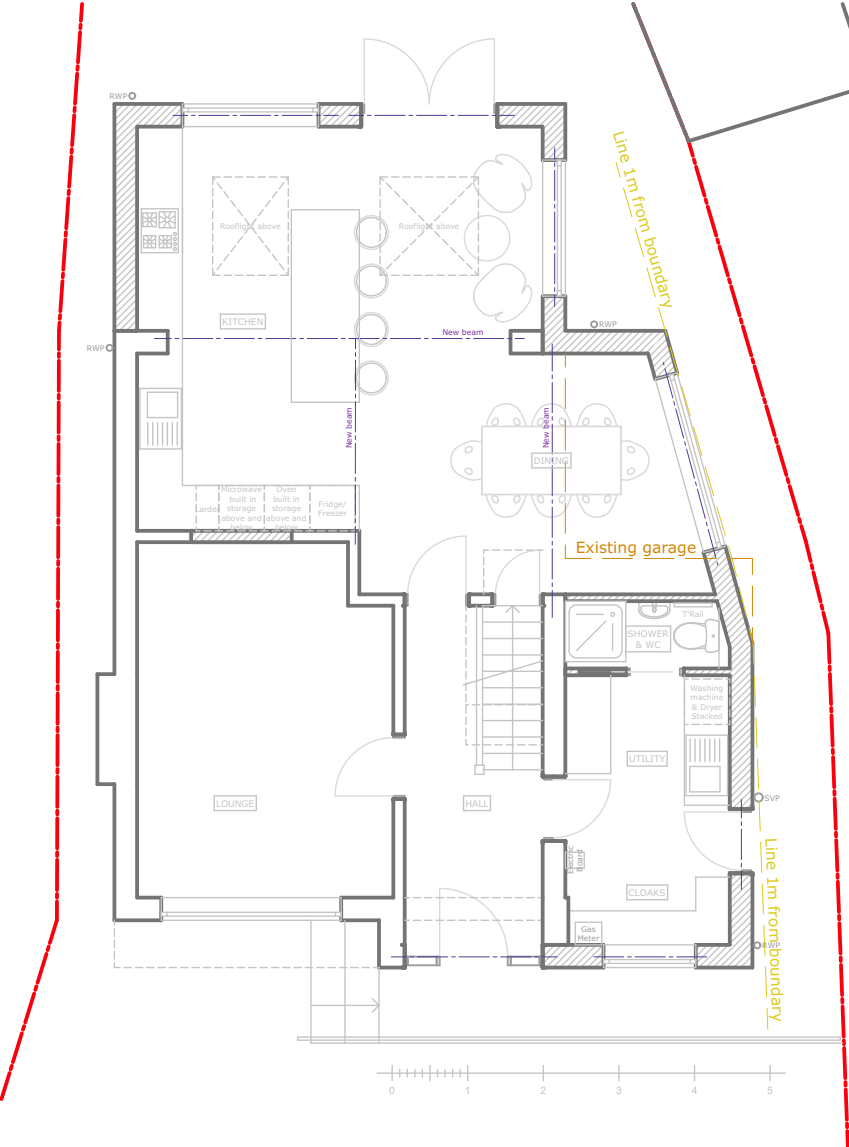
Ground Floor
