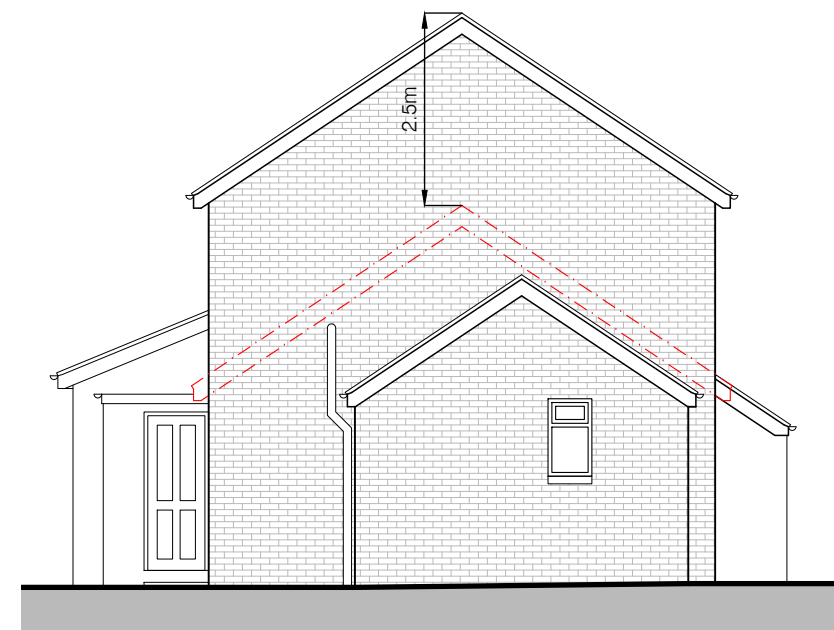
WEST ELEVATION - 1:100
