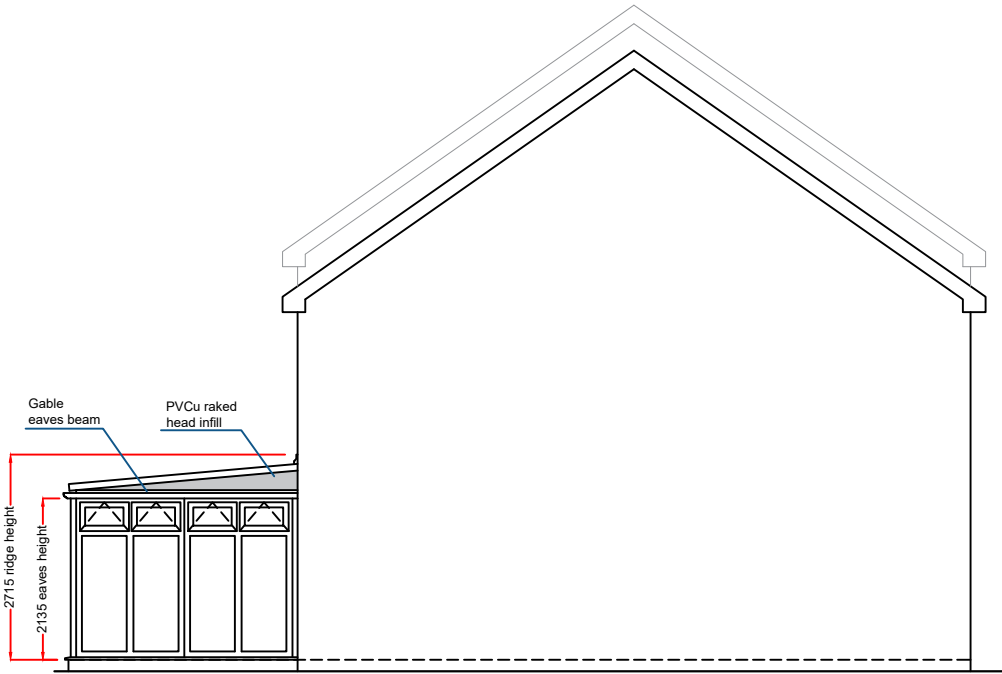
RIGHT-HAND SIDE ELEVATION
