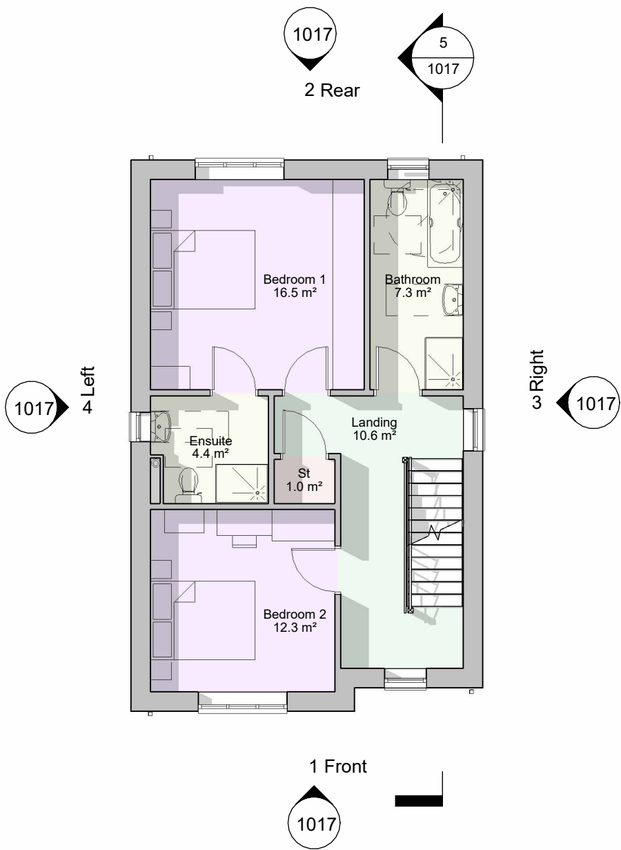
First Floor 1 : 100
