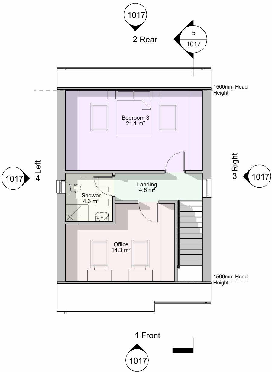
Second Floor 1 : 100
