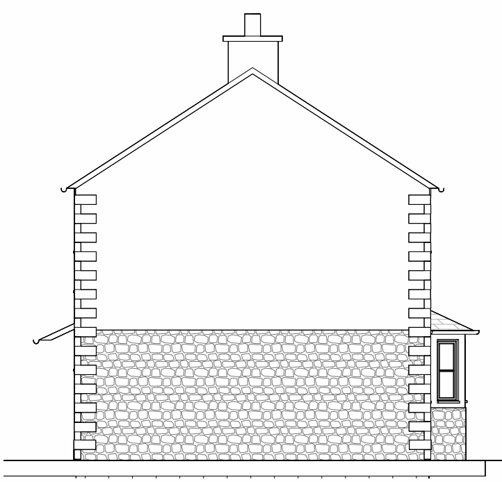
Side - North 1 : 100
