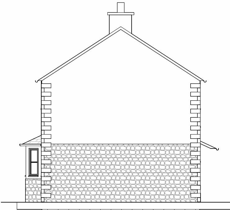
Side - South 1 : 100
