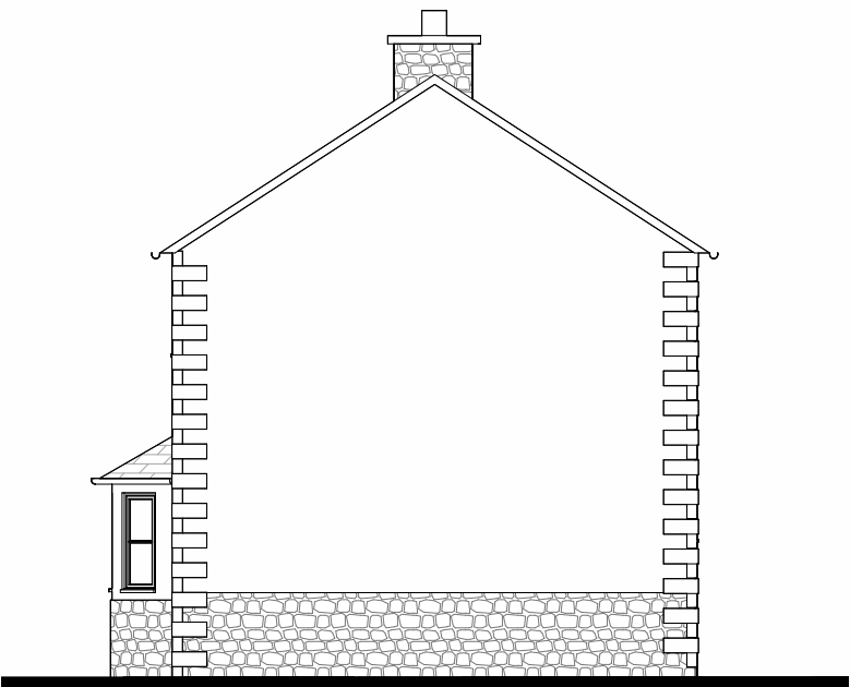
Side - South
