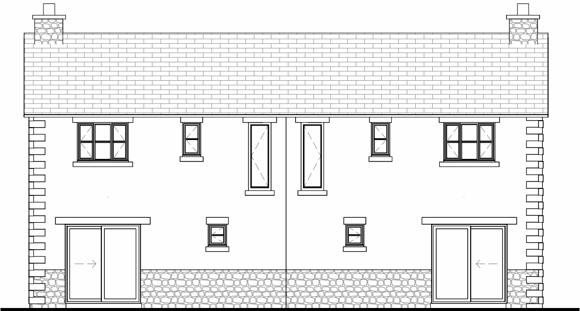
Rear - East
