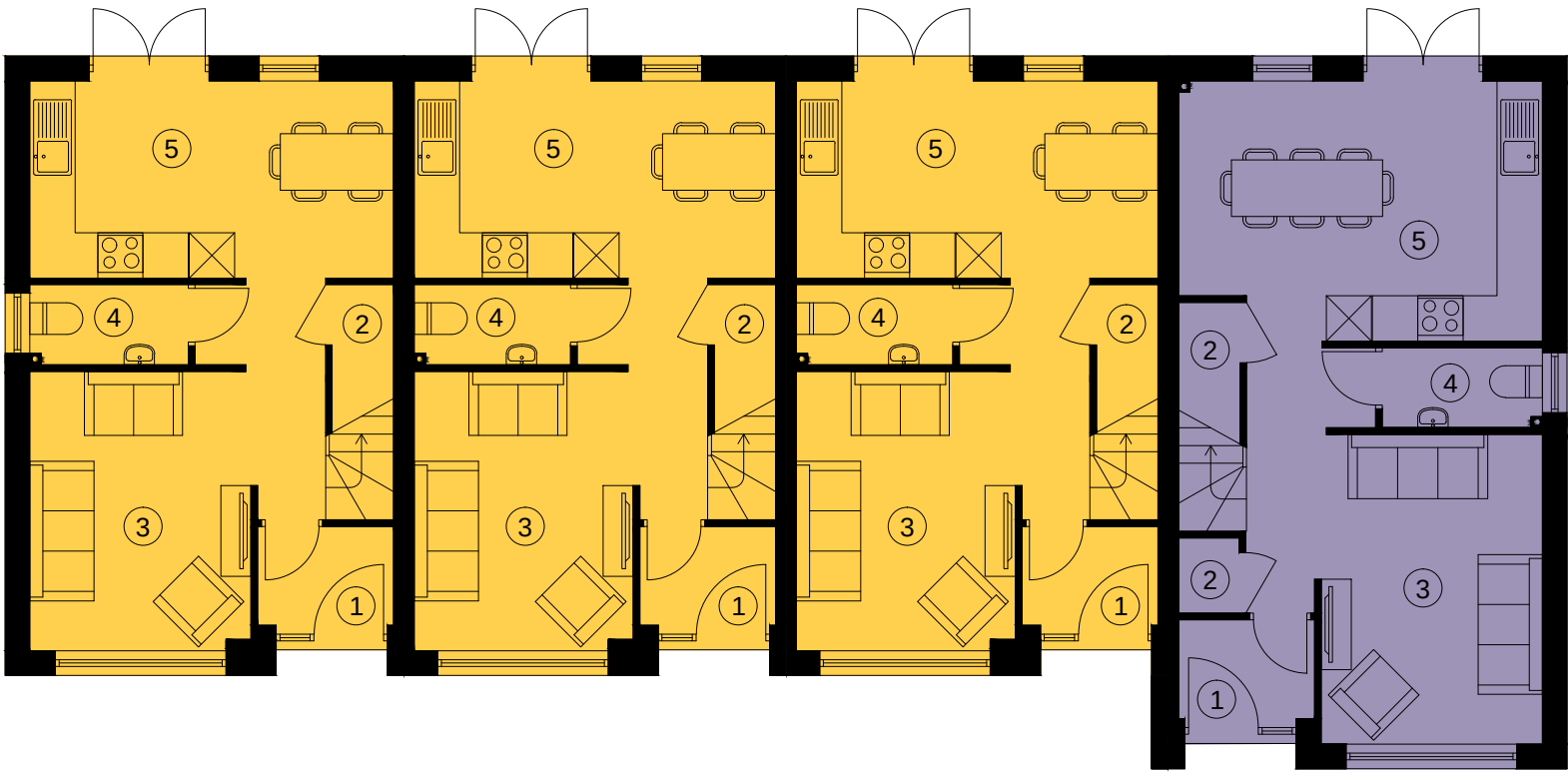
Ground floor
