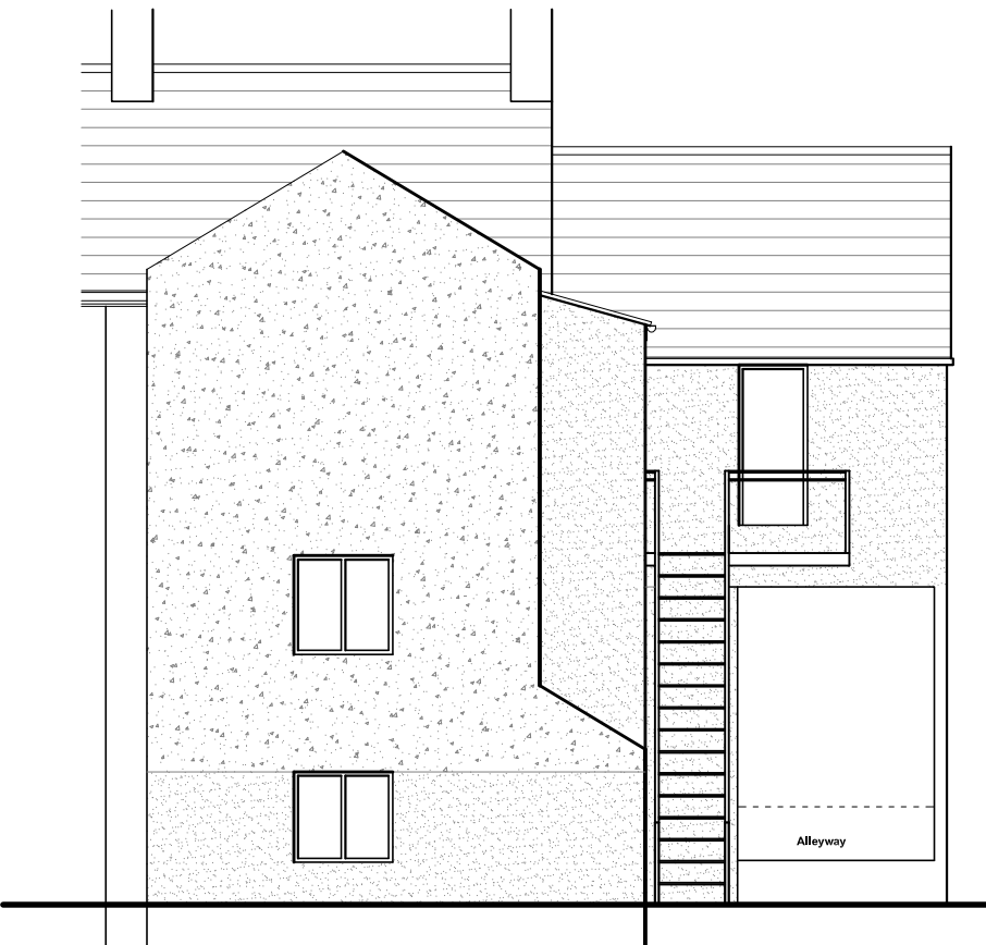
Rear Elevation - West
