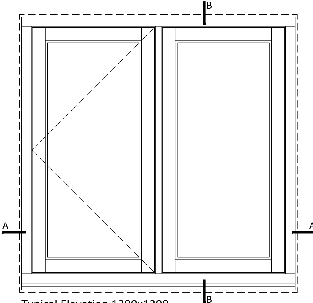
Typical Elevation 1200x1200
