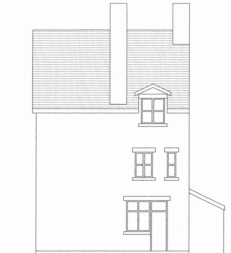
ELEVATION TO EAST
