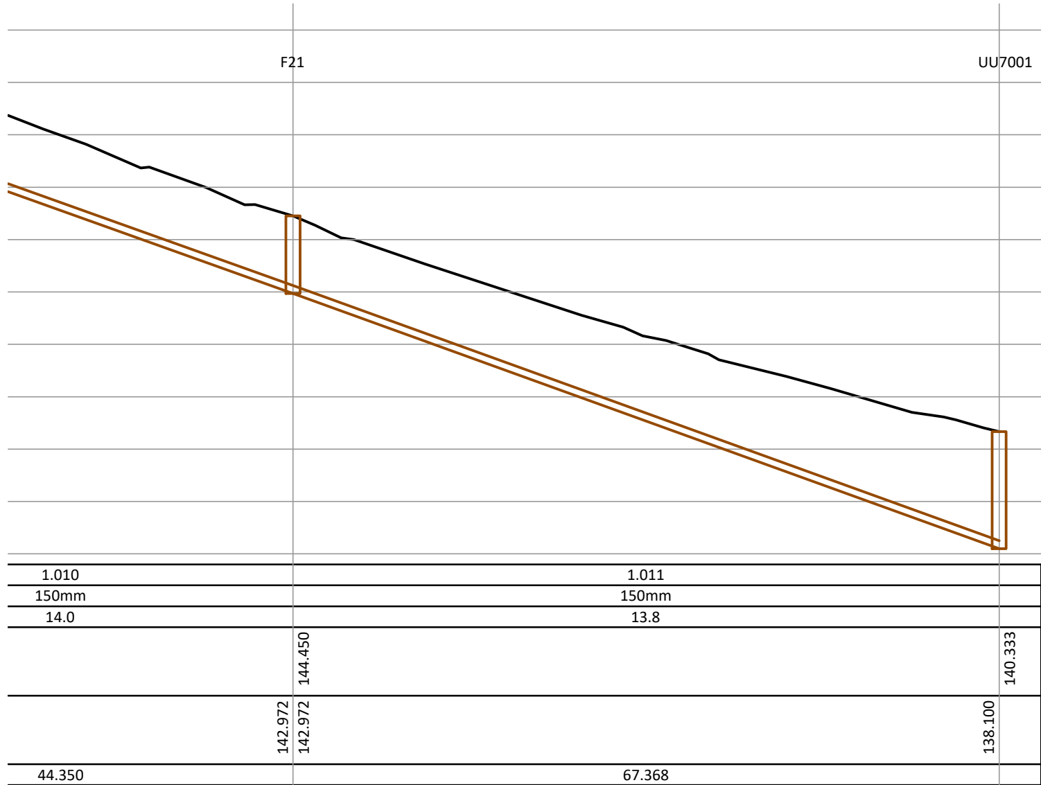
Foul Water Drainage Longitudinal Section - Run 01 Continued Horizontal Scale 1:500 Vertical Scale 1:100
