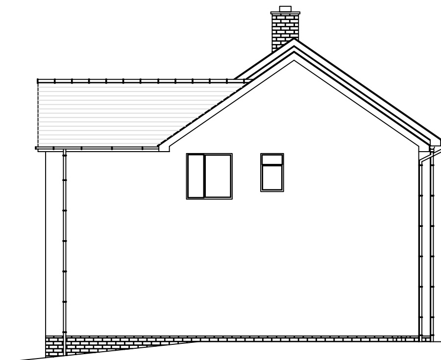
Side Elevation (Existing / Proposed)
