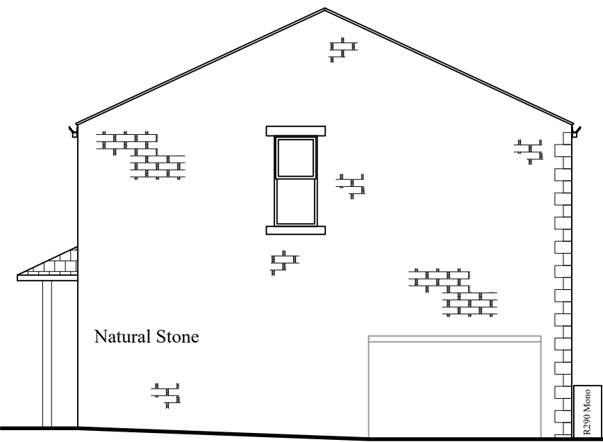
North (Side)
