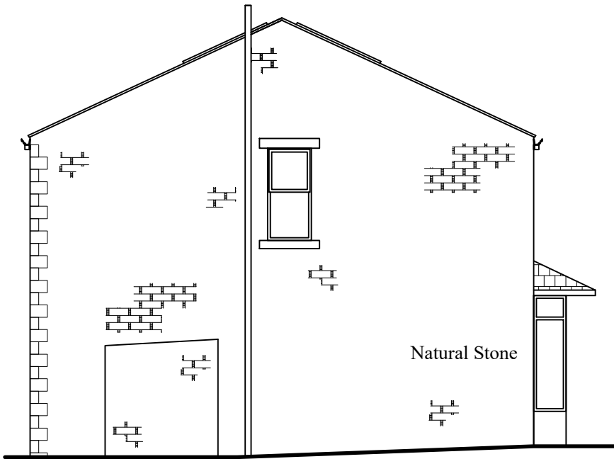
South (Side)
