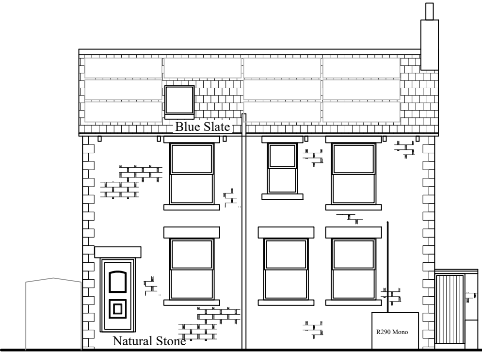
West (Rear)
