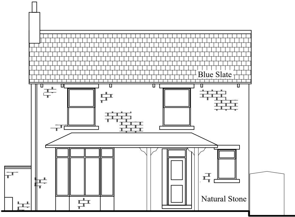
East (Front)
