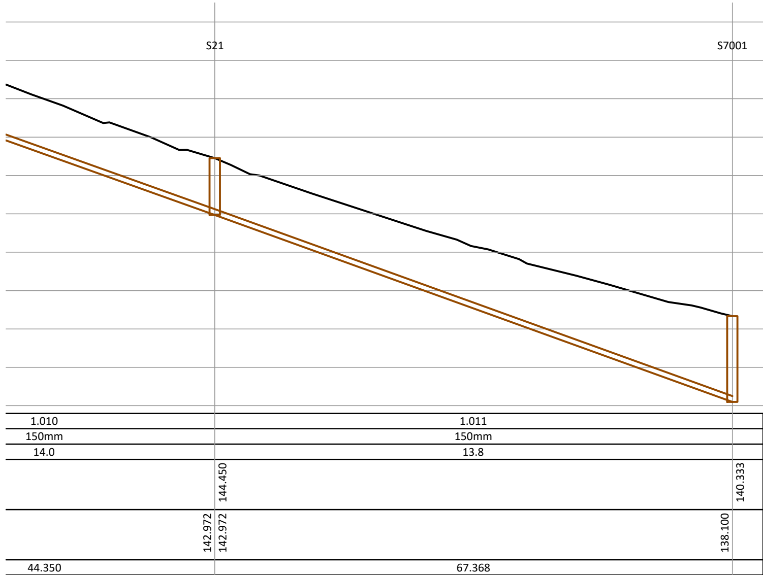
Foul Water Drainage Longitudinal Section - Run 01 Continued
