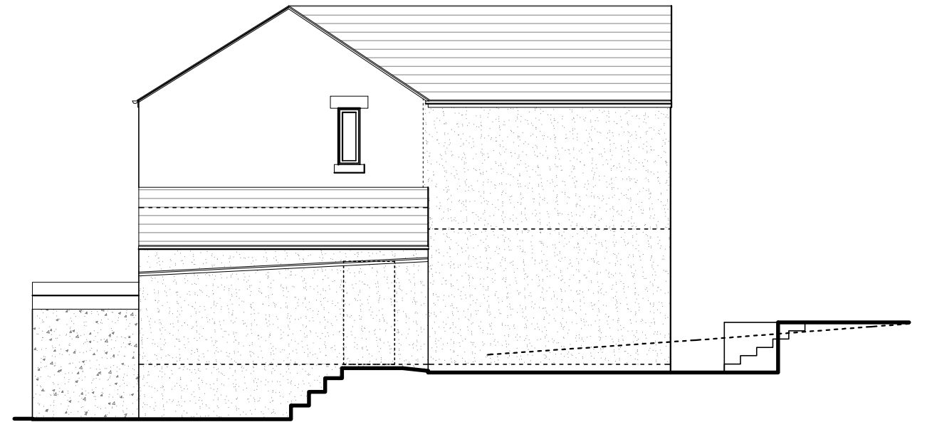
Side South West Elevation
