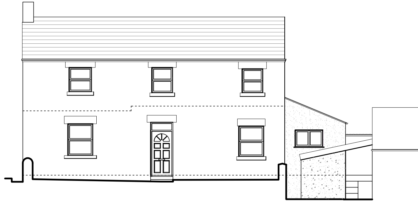
Front North West Elevation
