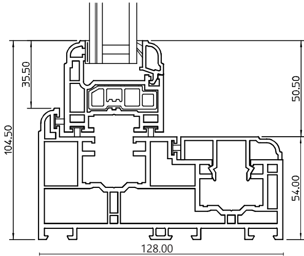
Top Rail
