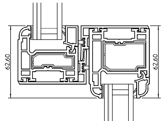
Meeting Rail
