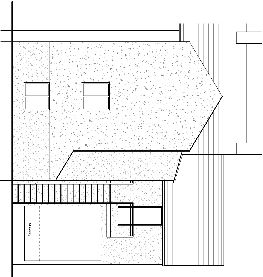
Rear Elevation - West
