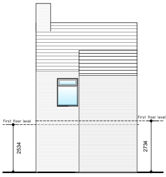
REAR ELEVATION BB 1:200
