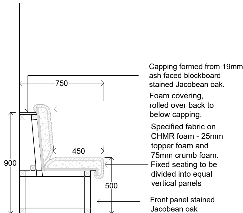
FS05 - FIXED SEATING SECTION SCALE 1:20
