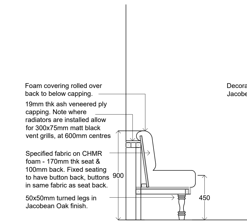
FS04 - FIXED SEATING SECTION SCALE 1:20
