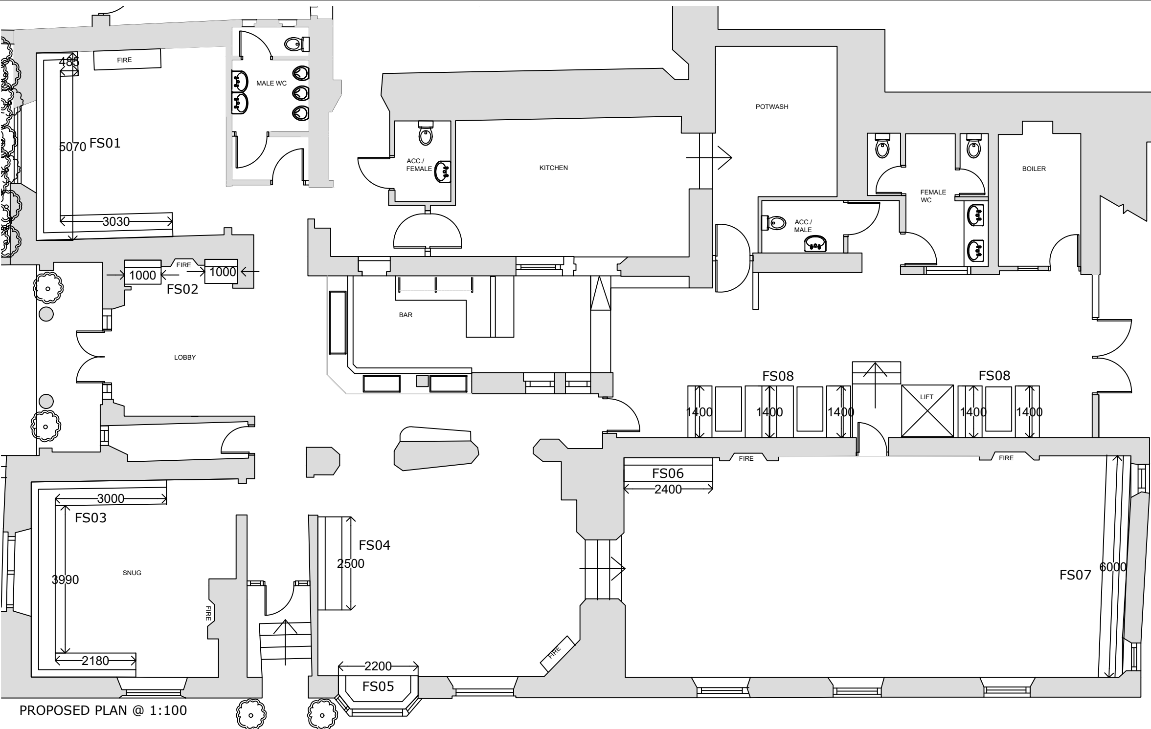
PROPOSED PLAN @ 1:100
