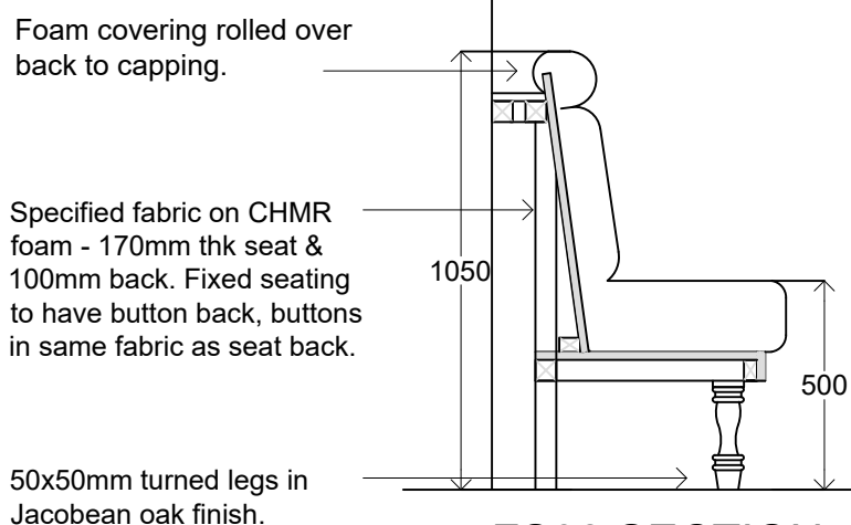
FS08 SECTION SCALE 1:20
