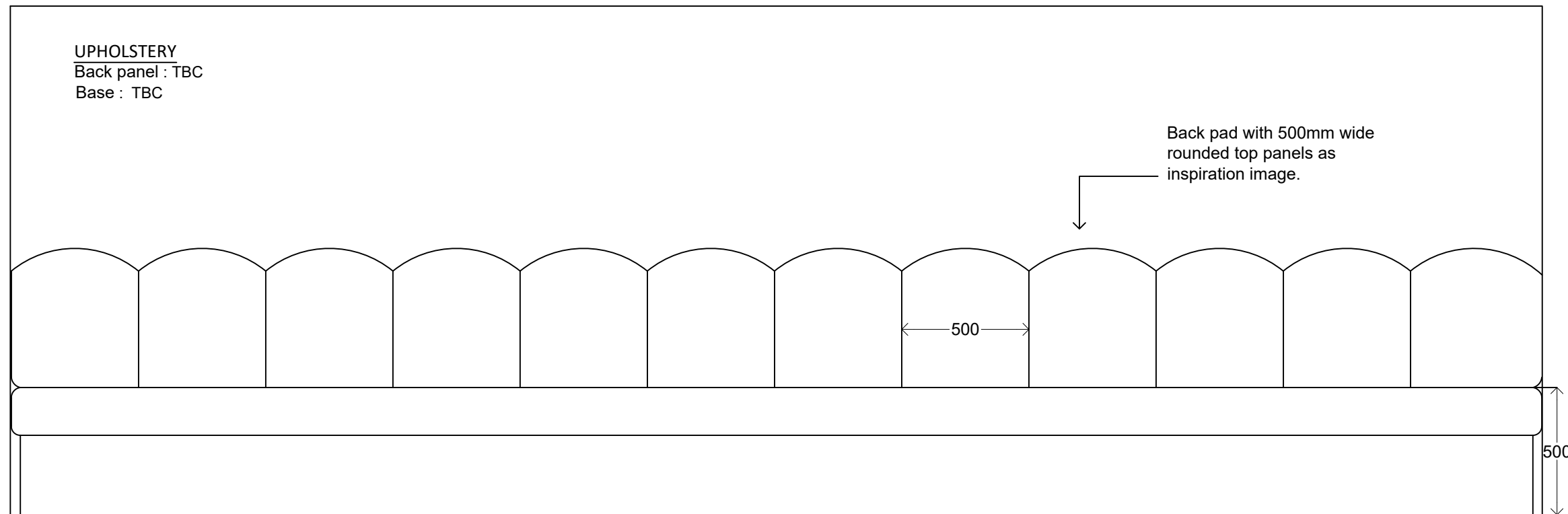
FS07- FIXED SEATING SCALE 1:20
