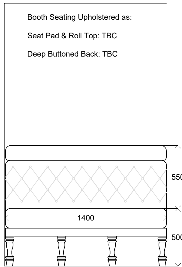
FS08- FIXED SEATING SCALE 1:20
