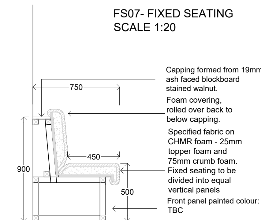
FS07 SECTION SCALE 1:20
