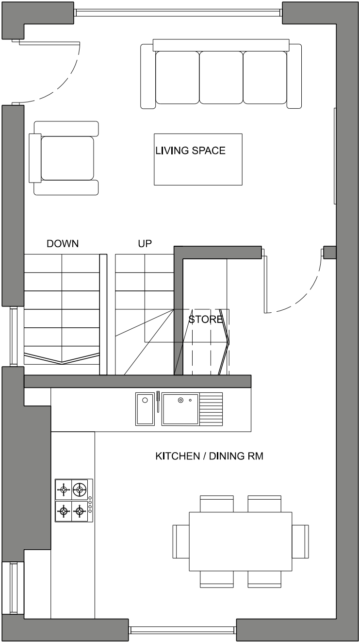
GROUND FL LEVEL
