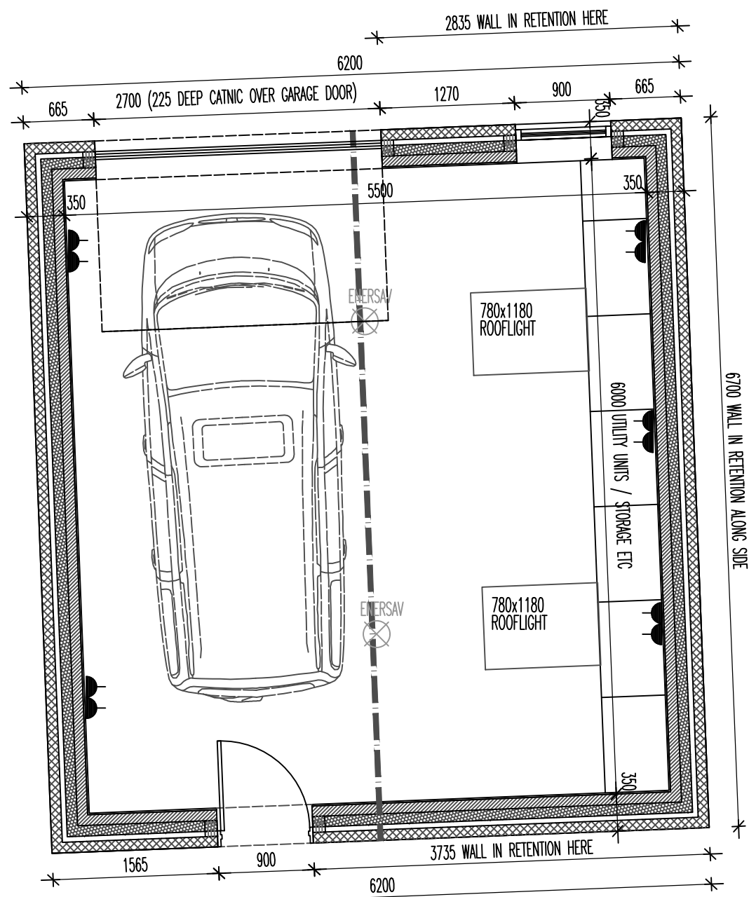
GROUND 1:50
