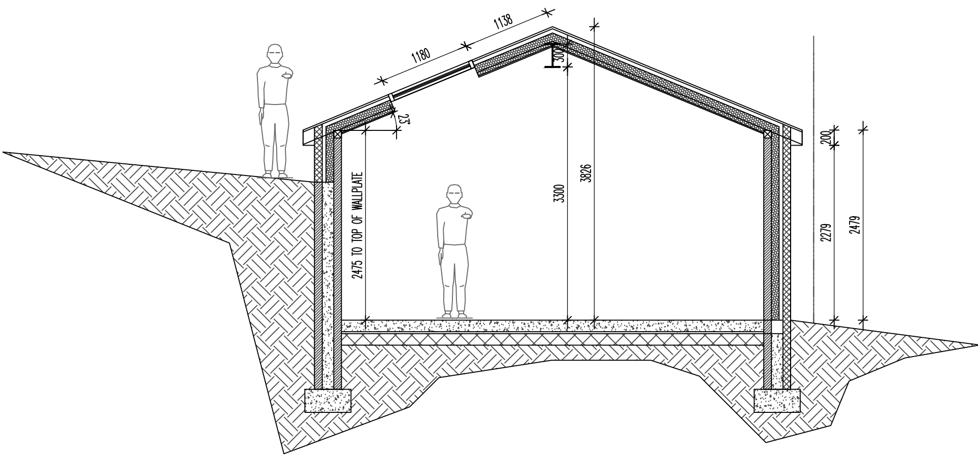
SECTION 1:50
