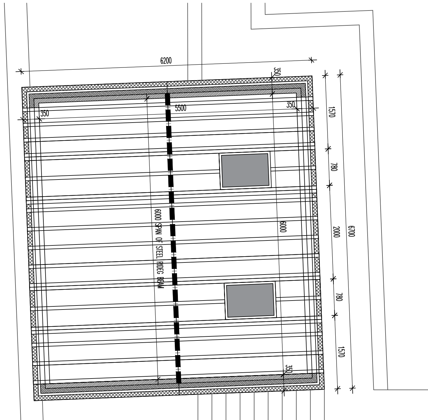
RAFTER PLAN 1:50
