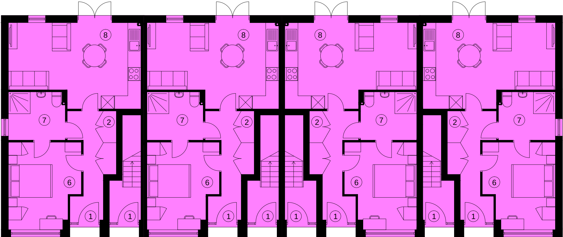
Ground floor
