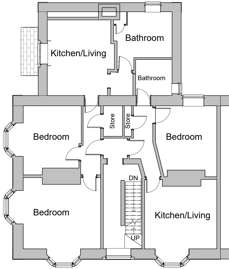
First Floor FFL Existing 1 : 100
