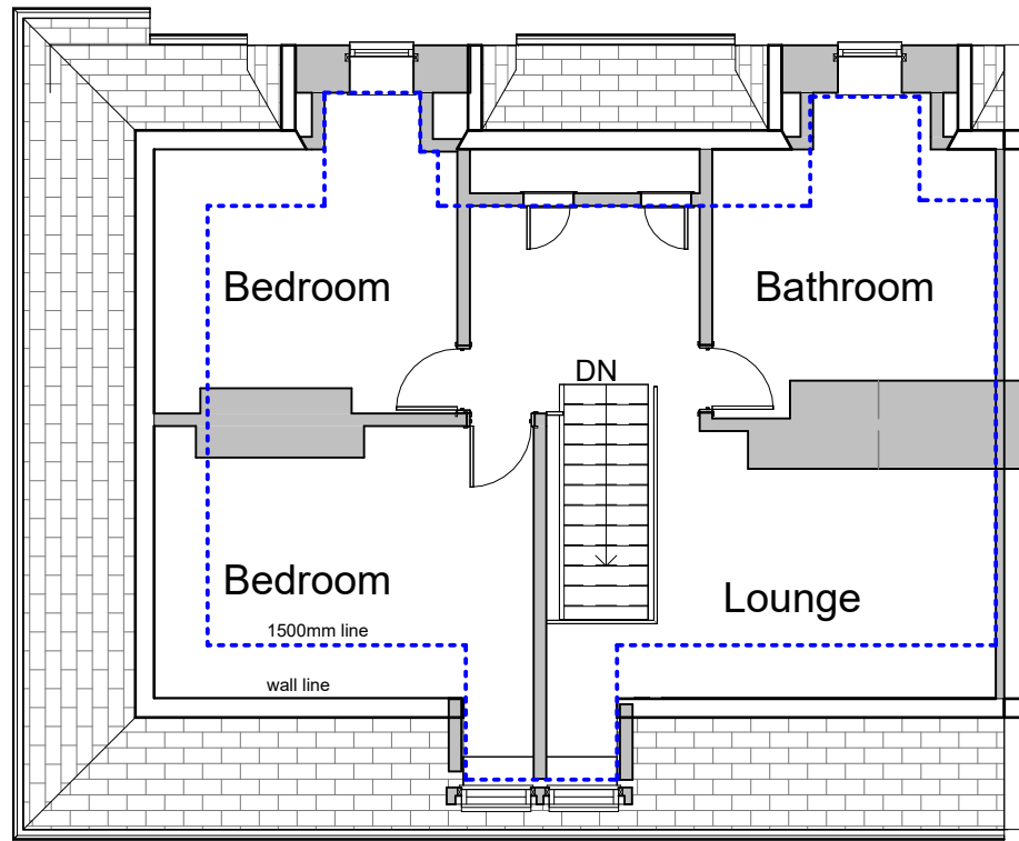
Third Floor FFL Existing 1 : 100
