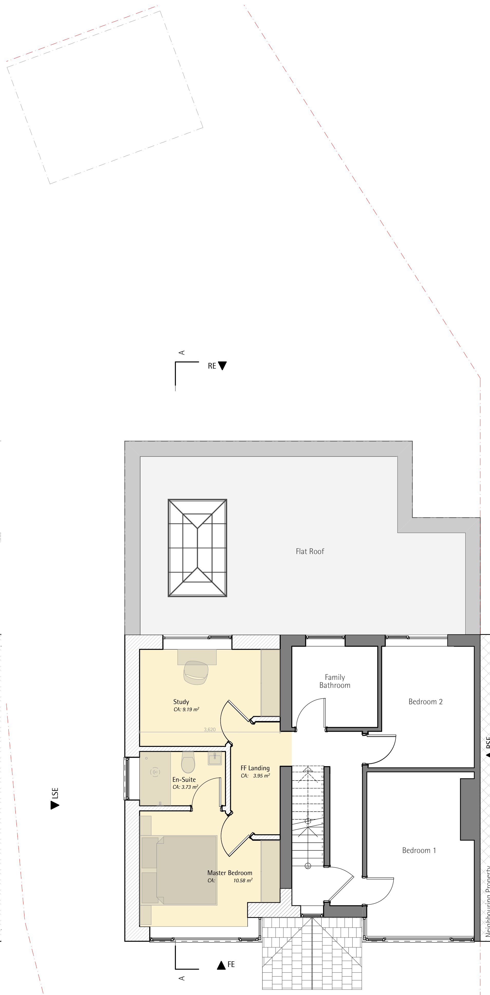
First Floor Plan (Proposed) 1:50
