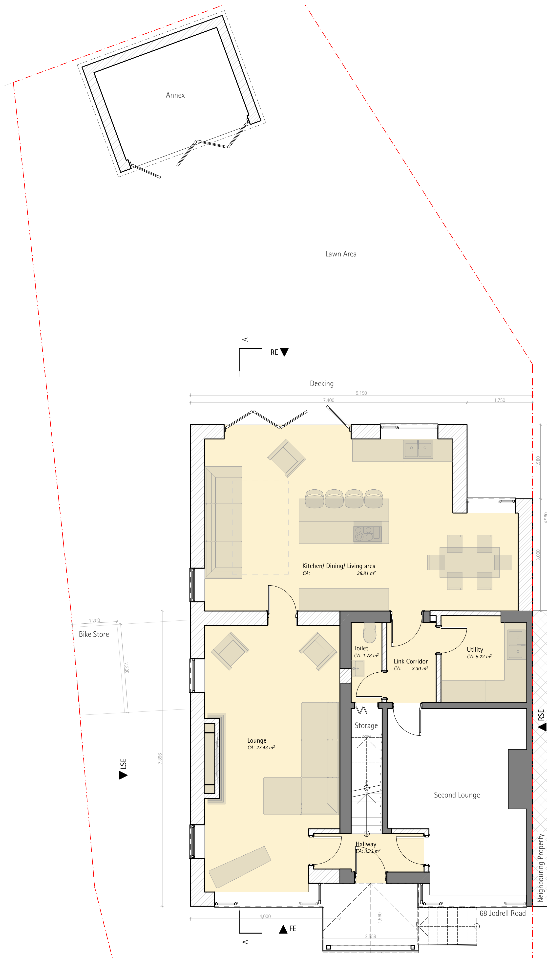
Ground Floor Plan (Proposed) 1:50
