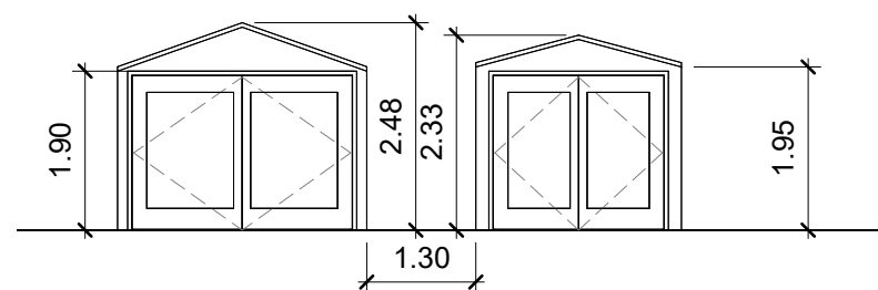
Front - West existing 1 : 100
