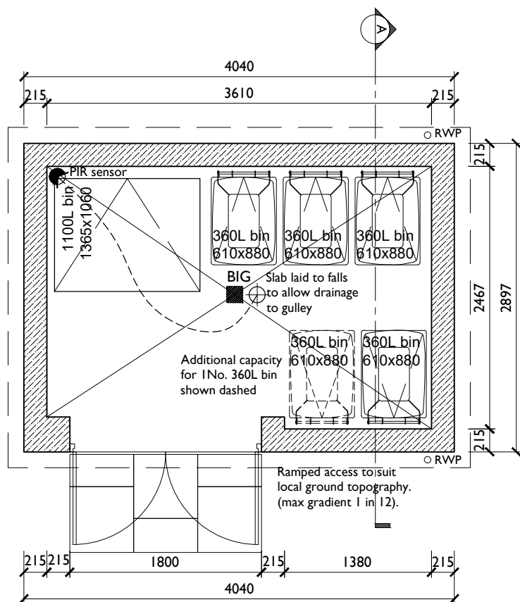
Ground Floor Layout 1:50
