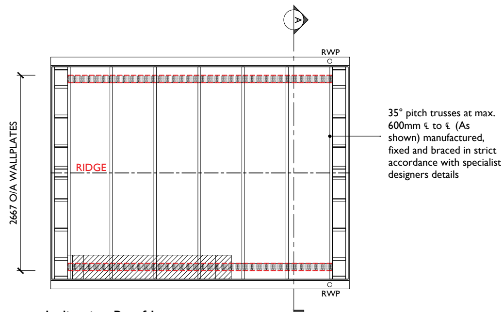
Indicative Roof Layout 1:50
