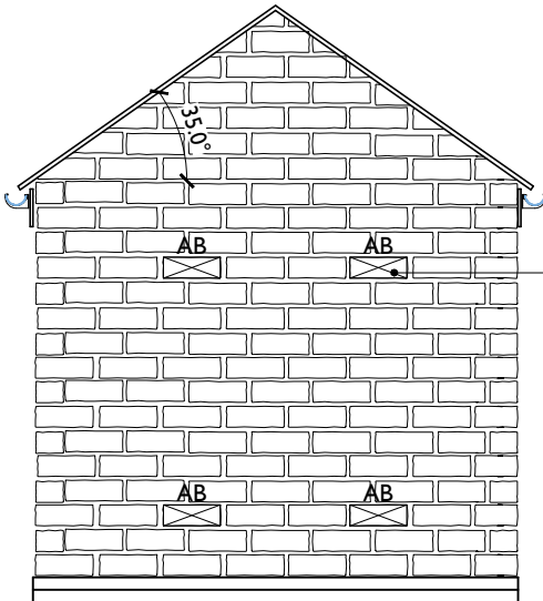
Side Elevation 1:50
