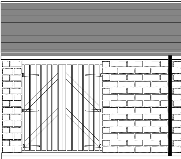
Front Elevation 1:50
