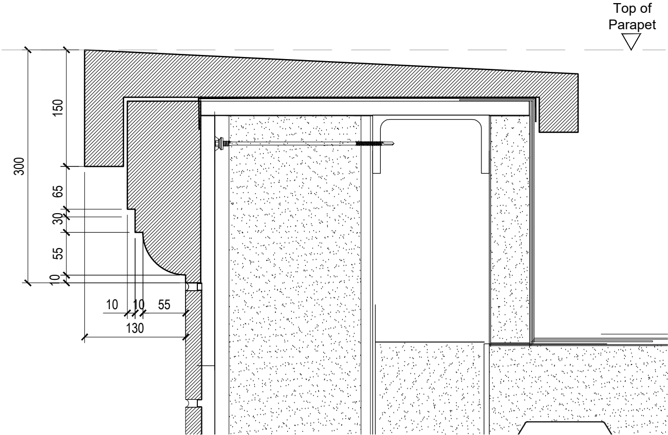
Proposed Cornice Profile
