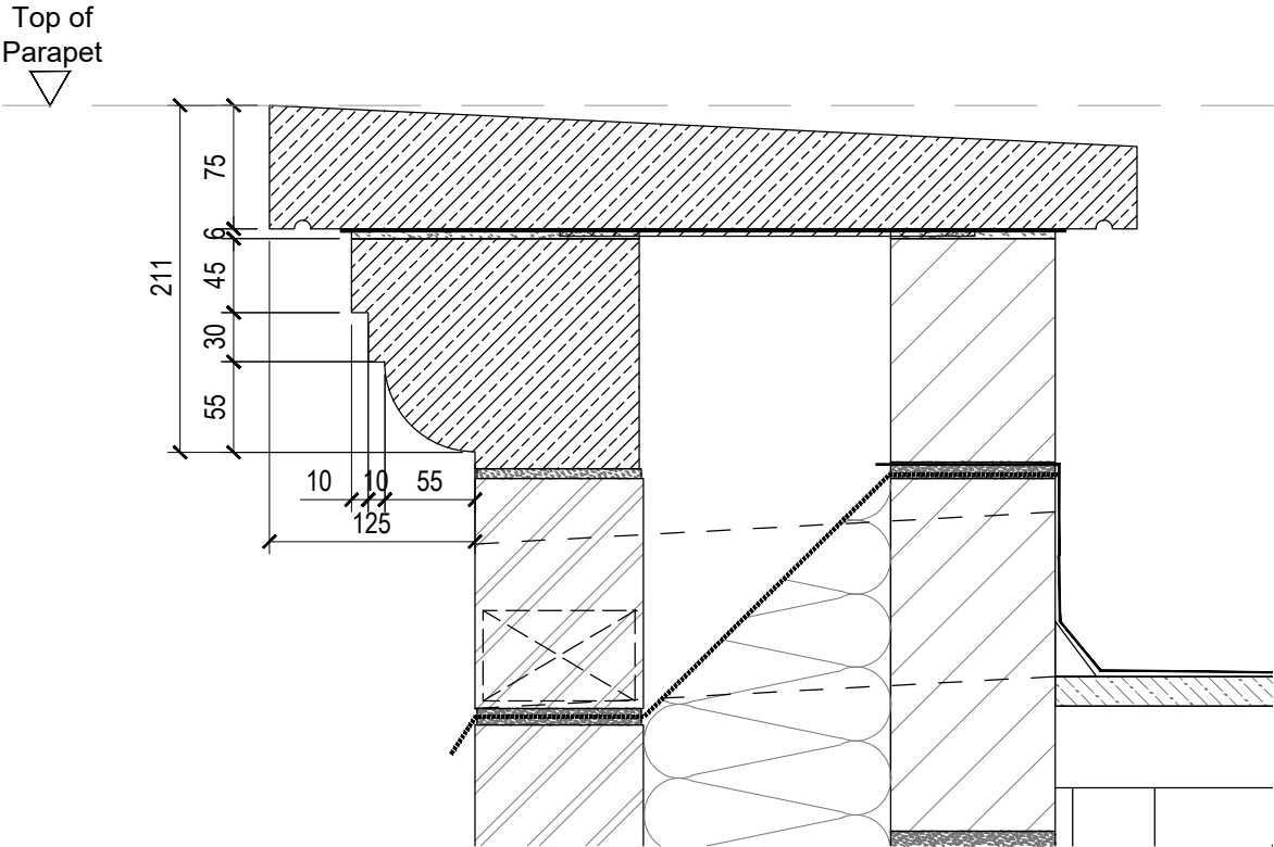
Existing McCarthy & Stone Cornice Profile (Drawing Based on: NW-2463-03-AC-121 Cornice Details Dated: November 2020)
