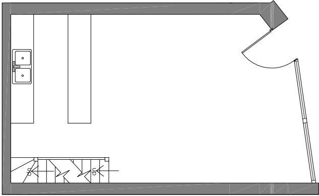
Existing and Proposed Ground Floor Plan
