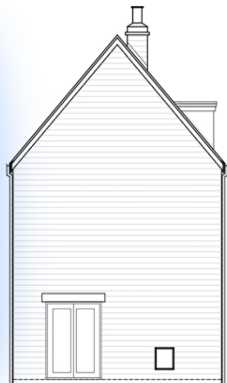
SIDE ELEVATION
