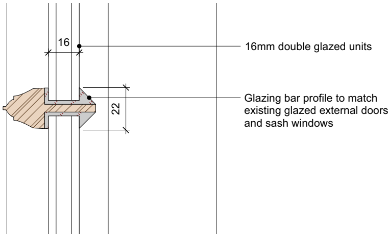
Glazing Bar Detail Scale - 1:2
