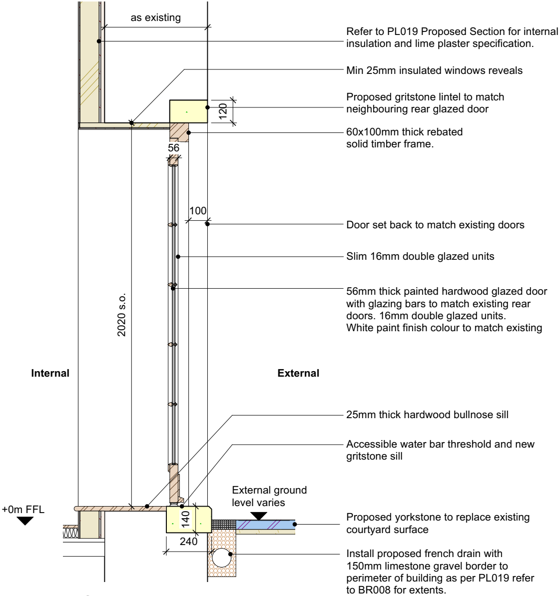
Window Section Detail Scale - 1:20
