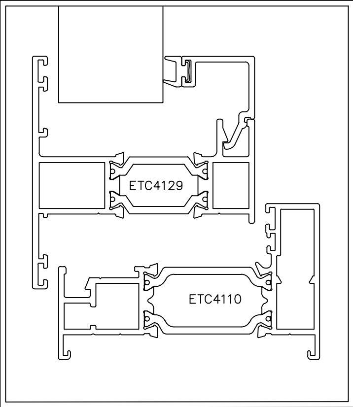
W1 Vertical Section (1:1)
