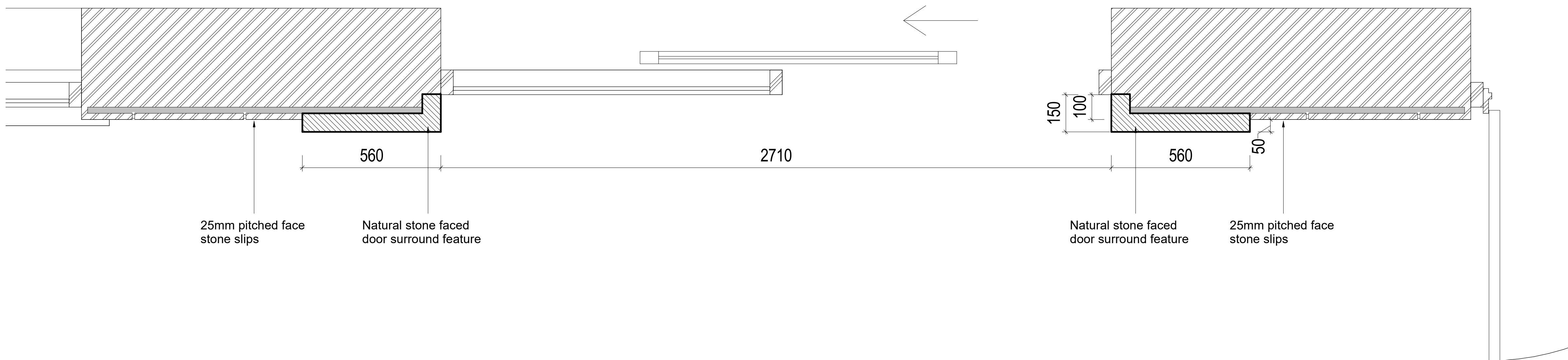
Entrance Plan Scale @ 1 : 10
