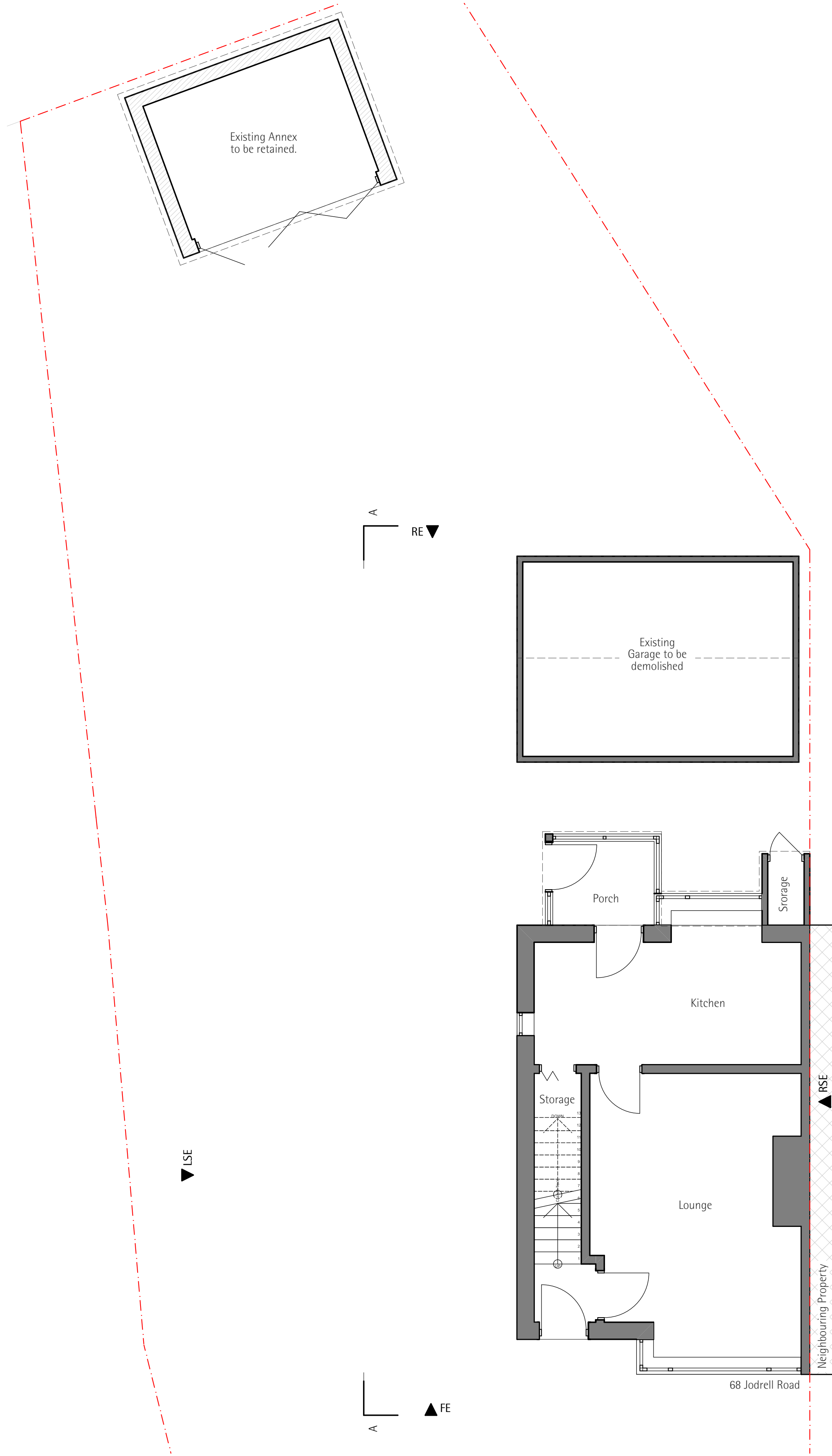
Ground Floor Plan (Existing) 1:50
