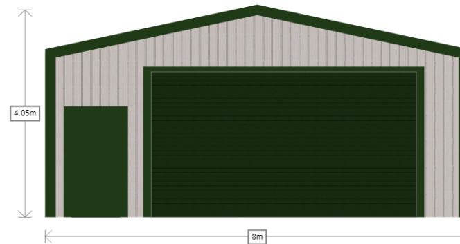
Right gable
