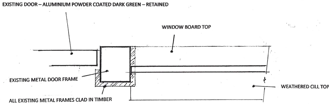
HORIZONTAL SECTION THROUGH DOOR FRAME SHOWING PROPOSED CLADDING (TO BE APPLIED TO ALL EXISTING FRAMES)
