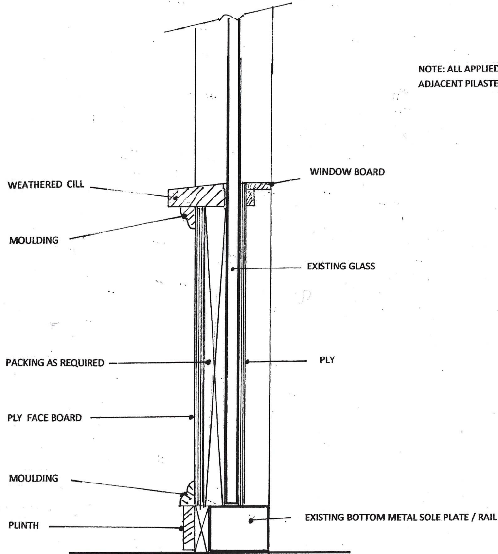
VERTICAL SECTION THROUGH PROPOSED STALL RISER
