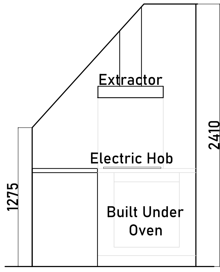
Section B-B. Kitchen Section Through Scale 1:20 @ A1
