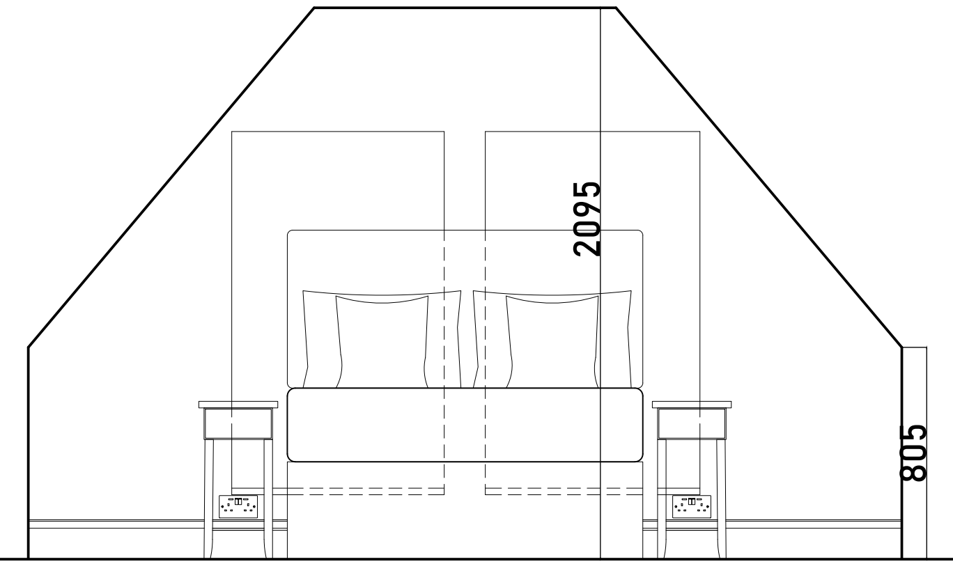
Section A-A. Bedroom Section Through Scale 1:20 @ A1
