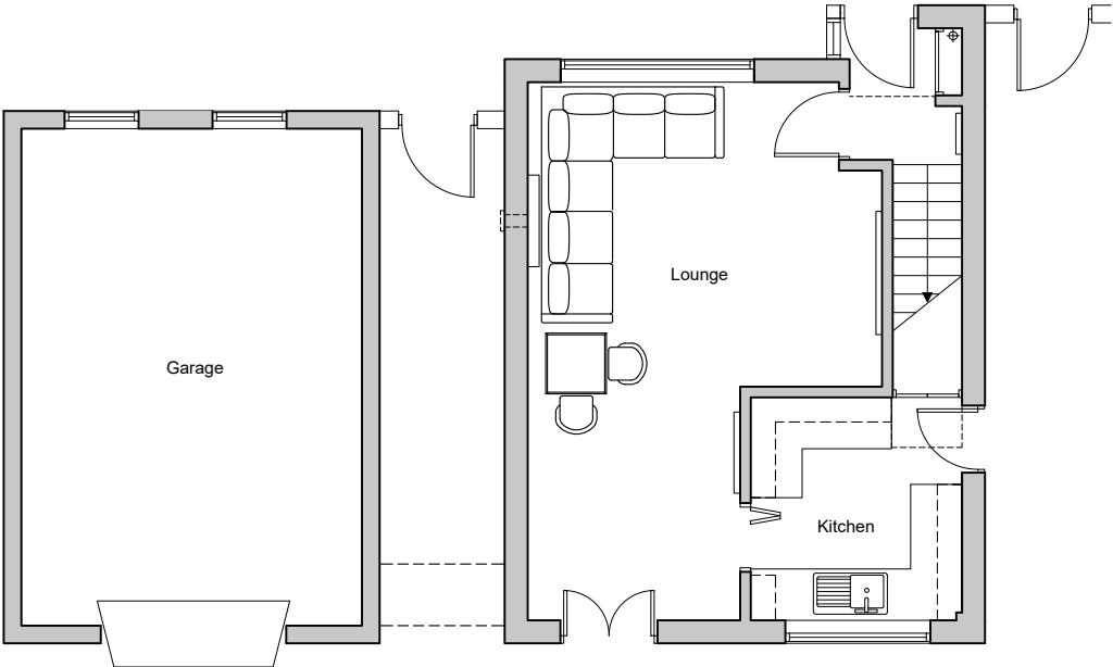
GROUND FLOOR: AS EXISTING 1:100
