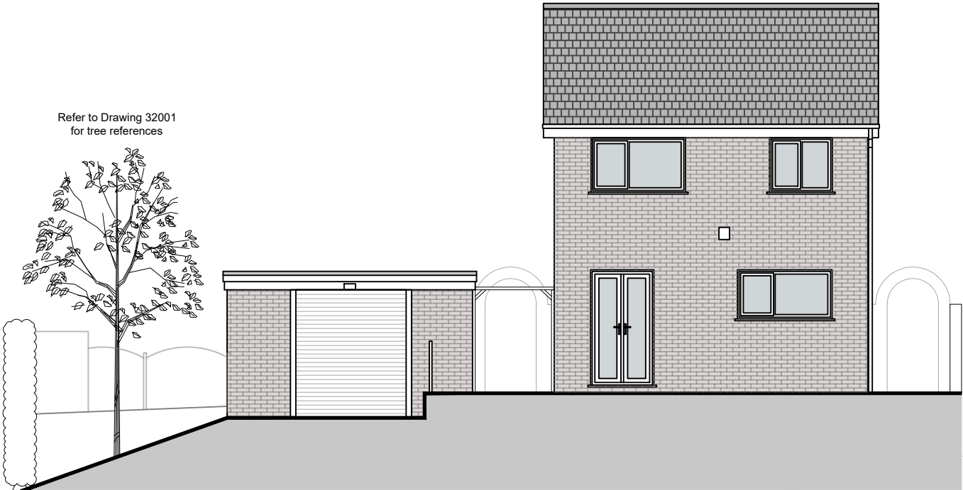
WEST ELEVATION: AS EXISTING 1:100
