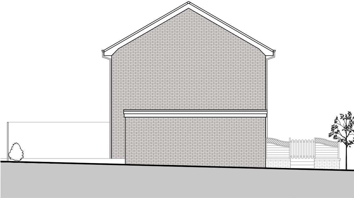
NORTH ELEVATION: AS EXISTING 1:100
