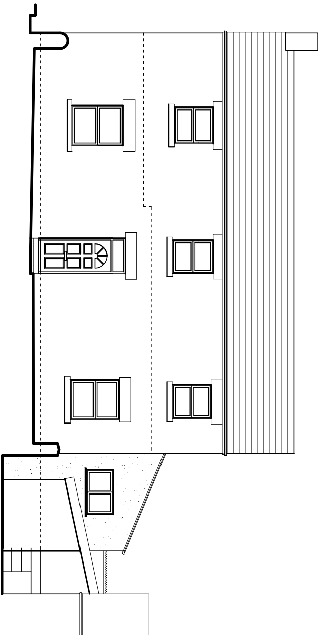
Front North West Elevation
