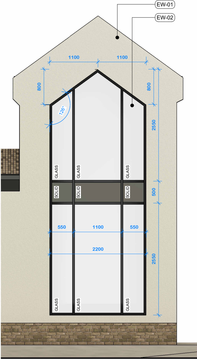
Proposed - Curtain Wall Elevation 1 : 50
