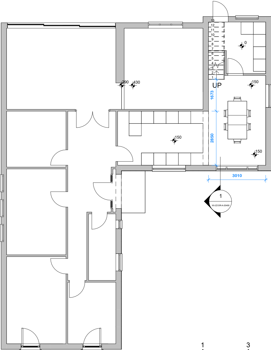
Level 0 - Proposed 1 : 100
