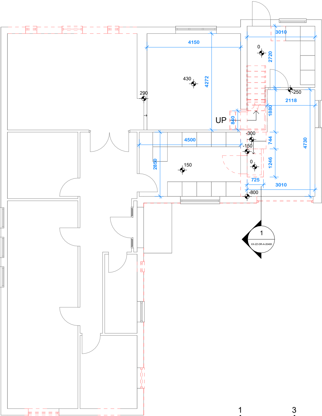
Level 0 - Existing and Demo 1 : 100
