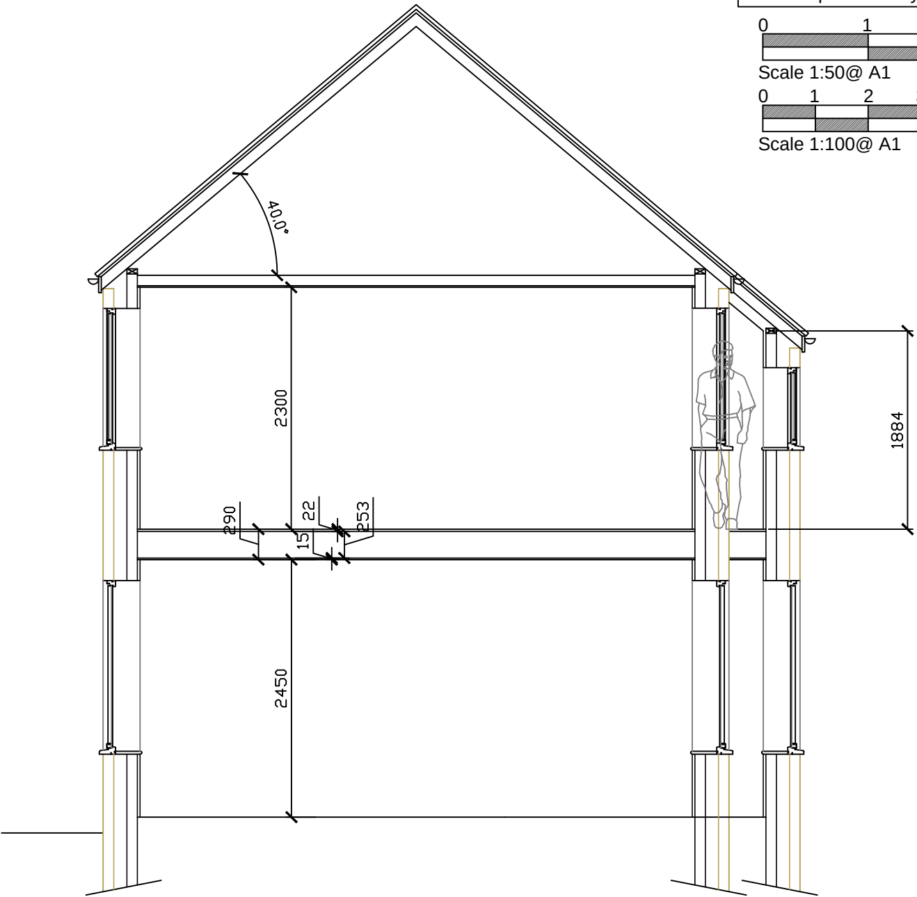
Proposed Sketch Section
