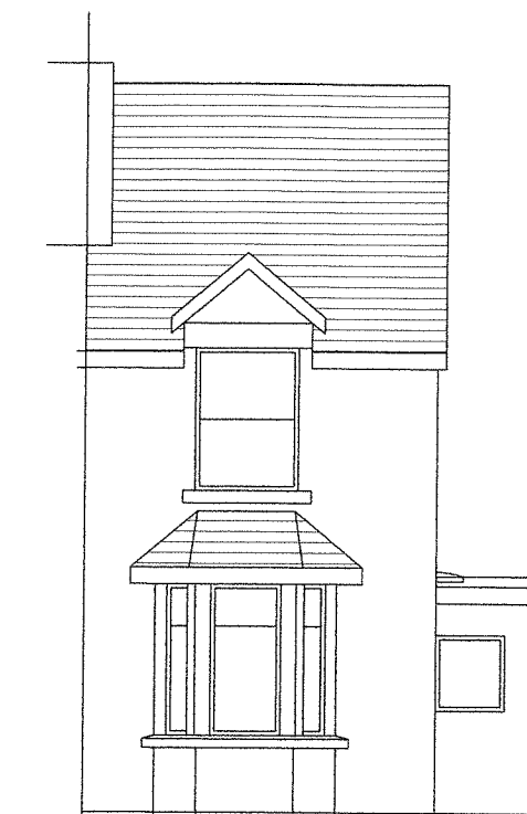
ELEVATION ON NEW WINDOW, porch not shown.
