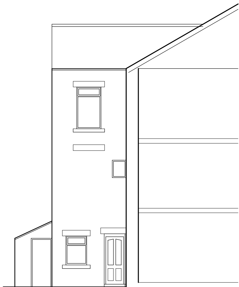
SECTIONAL SIDE ELEVATION
