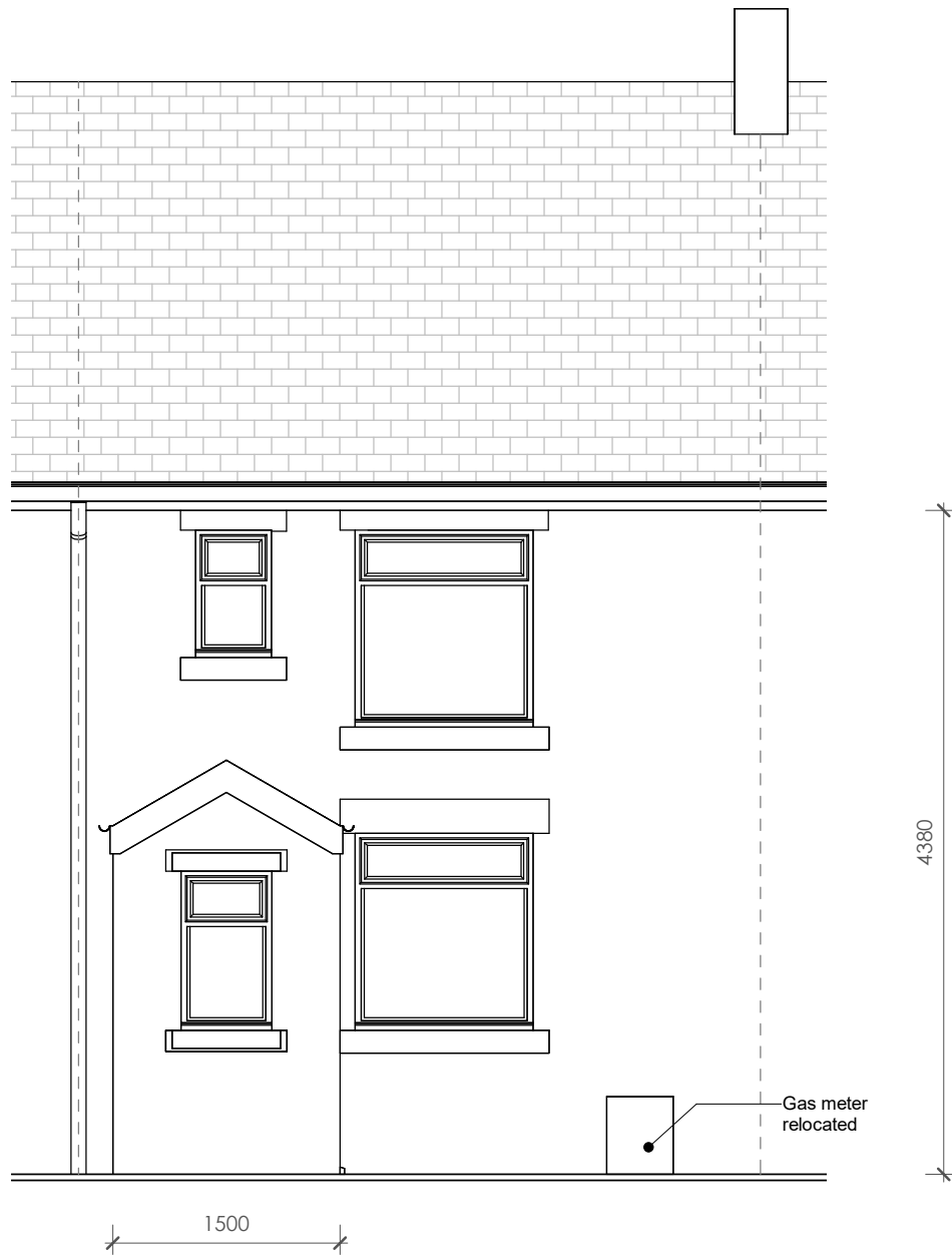
Proposed Front Elevation - Option 2 1 : 50
