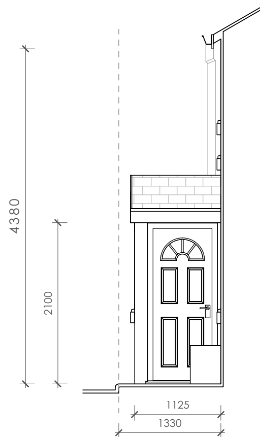
Proposed Side Elevation 1 : 50
