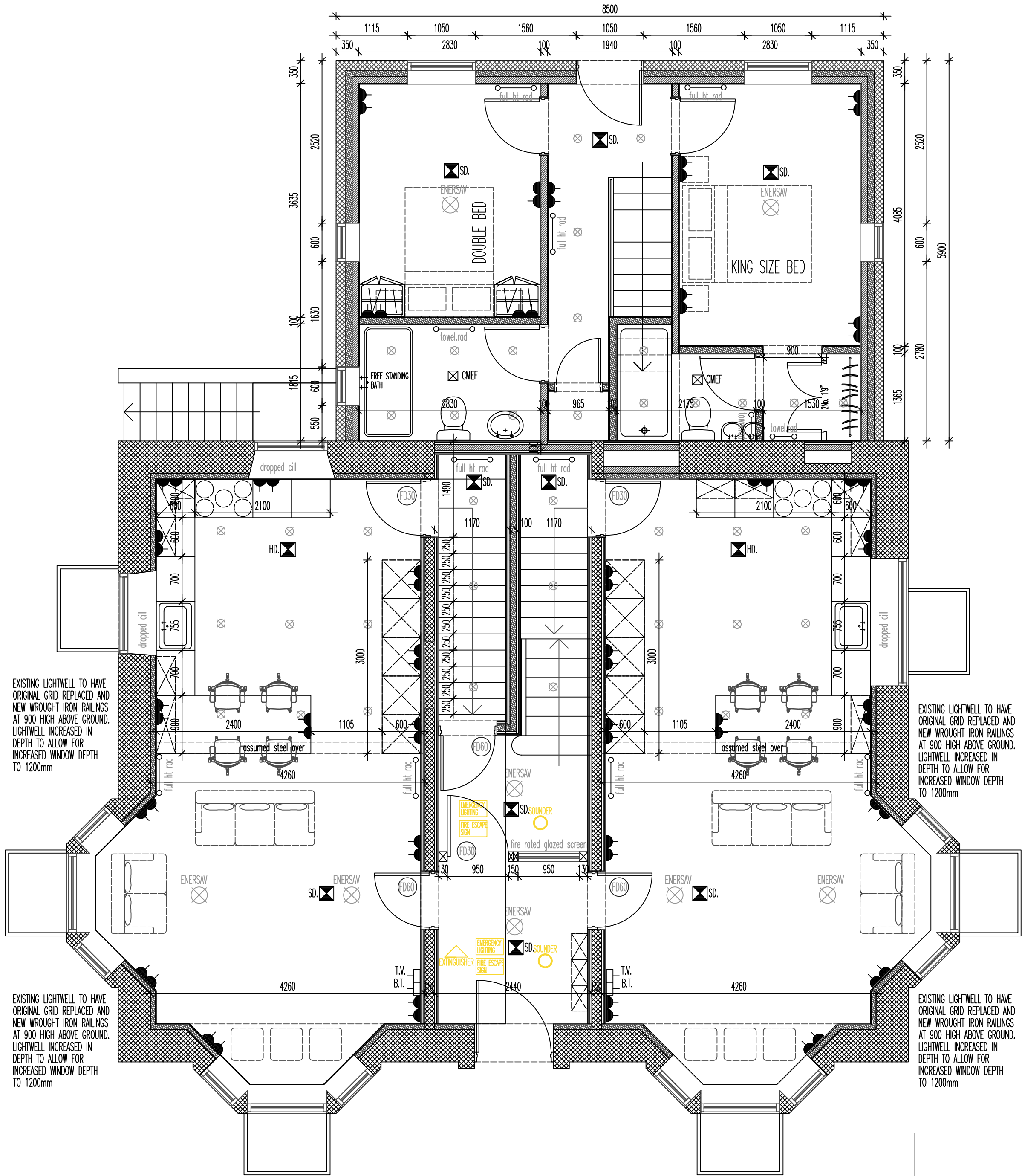
2 x 2 bed maisonette apartments: 92 M2
