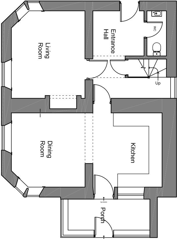
Main House Ground Floor
